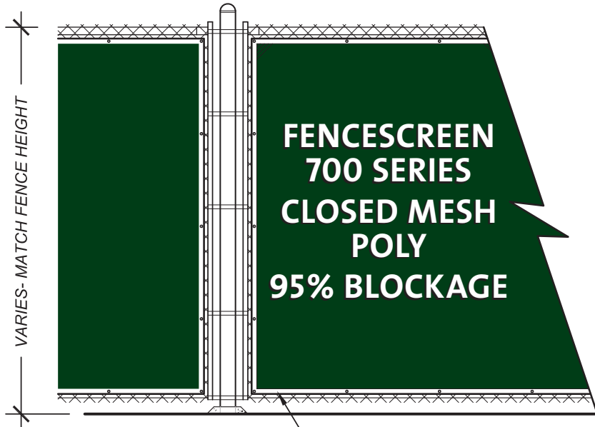
ELEVATION VIEW
