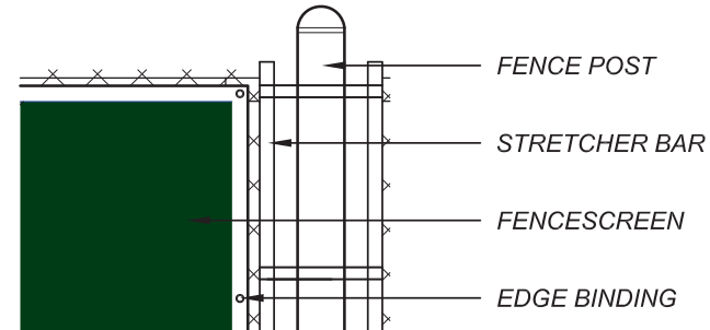
ATTACHMENT ENLARGEMENT
